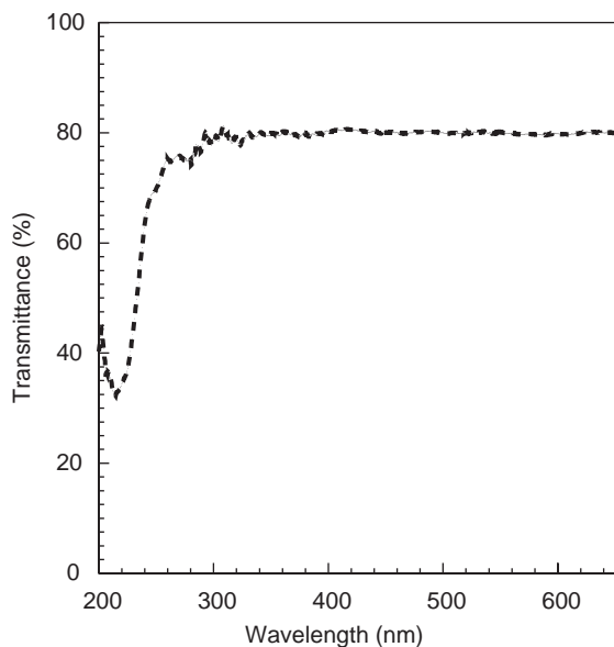
Fig. 3. Optical transmittance as a function of wavelength for \text{LaCl}_3 crystal (4 mm in thickness).
