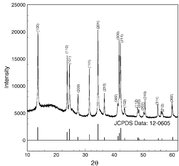
Fig. 2. XRD pattern of as-grown \text{LaCl}_3 crystal.
