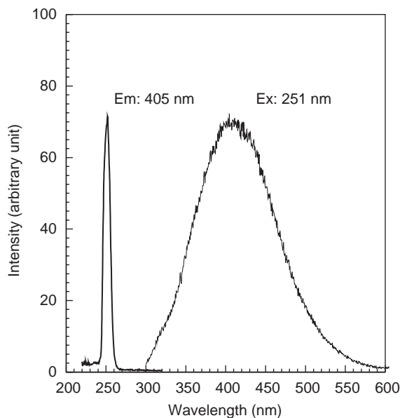
Fig. 4. Emission and excitation spectra as a function of wavelength for \text{LaCl}_3 crystal.
