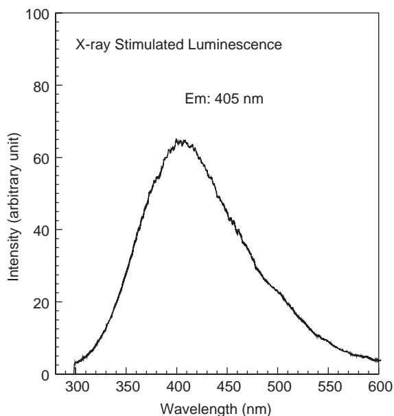
Fig. 5. X-ray stimulated luminescence spectrum as a function of wavelength for \text{LaCl}_3 crystal.
