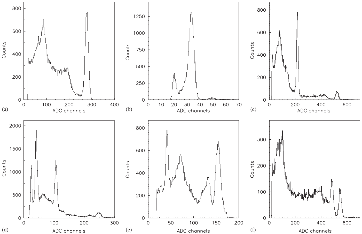
Fig. 5. Energy distributions measured by the \text{LaCl}_3\text{:Ce} detector with the PMT coupled to the optical window of the detector through the light guide by using the following \gamma sources: (a) ^{137}\text{Cs} with peak at 662 keV; (b) ^{241}\text{Am} with peak at 59.5 keV; (c) ^{22}\text{Na} with peaks at 511 and 1275 keV; (d) ^{228}\text{Th} with peaks at 239 and 583 keV (sources ^{228}\text{Th} set at \sim 10 cm from the detector); (e) ^{133}\text{Ba} with peaks at 81 and \sim 356 keV, in this case the source was positioned in a slightly different way than in the other cases; (f) ^{60}\text{Co} with peaks at 1173 and 1332 keV.
