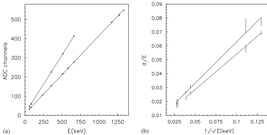
Fig. 6. (a) Linearity of the \text{LaCl}_3\text{:Ce} crystal, without (upper line) and with (lower line) light guide. The points correspond to the \gamma photopeaks in the Fig. 4 for the calibration without light guide and in Fig. 5 for the calibration with light guide. (b) Behaviours of \sigma/E measured with the \text{LaCl}_3\text{:Ce} detector without (lower line) and with (upper line) light guide, respectively; in the case with light guide only 7 of the 10 \gamma peaks present in Fig. 5 have been considered. In fact, for ^{228}\text{Th} peaks the source was at \sim 10 cm from detector, while the peak at \sim 356 keV from ^{133}\text{Ba} is due to the superimposition of more \gamma 's. In the case without light guide only 4 peaks of Fig. 4 have been taken into account not considering for the same reason the \sim 356 keV peak from ^{133}\text{Ba} .
